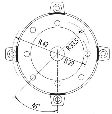
Fixing layout
